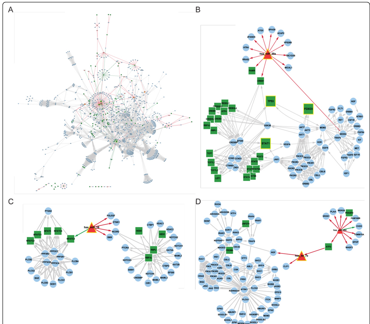
Figure 4 Differential regulatory network and key miRNA regulators of HCC metastasis. (A). Differential regulatory network of the 17 classifying modules and their enriched pathways. The green edges represent edges whose CLR weights are larger in network of non-metastasis, while the orange ones represent edges whose weights are larger in network of metastasis. The color and shape of the nodes represent the type of "genes": TF in green rectangle, miRNA in red triangle, and gene in blue ellipse. Six regulators of which modules were enriched in KEGG non-metabolic pathways are highlighted in nodes with larger size and yellow border (hsa-miR-16, hsa-miR-30a, hsa-let-7e, STAT1, TP53, FOXO3). The graph structure of KEGG pathways embodied by gene(protein)-gene(protein) interactions was retrieved by the R package KEGGgraph. (B). Differential regulatory network of miR-30a. (C). Differential regulatory network of miR-16. (D). Differential regulatory network of let-7e/miR-204.
