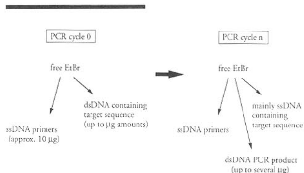
FIGURE 1 Principle of simultaneous amplification and detection of PCR product. The components of a PCR containing EtBr that are fluorescent are listed—EtBr itself, EtBr bound to either ssDNA or dsDNA. There is a large fluorescence enhancement when EtBr is bound to DNA and binding is greatly enhanced when DNA is double-stranded. After sufficient (n) cycles of PCR, the net increase in dsDNA results in additional EtBr binding, and a net increase in total fluorescence.
